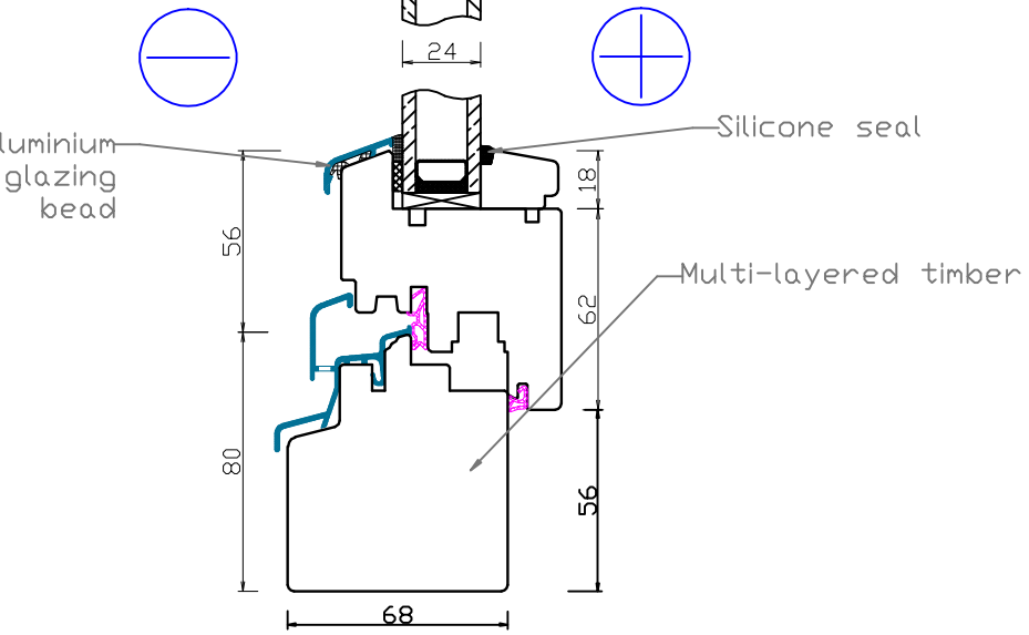
STANDRAD FLUSH SILL
