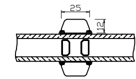
25mm Glazing Bar
