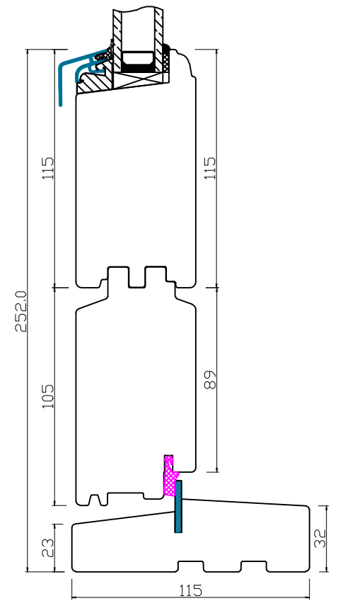
FLUSH HARDWOOD SILL
