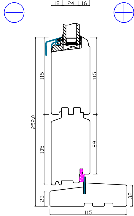
FLUSH HARDWOOD SILL
