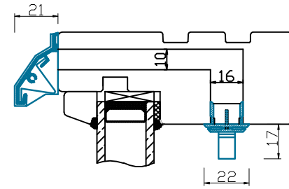
TRICKLE AIR VENT
