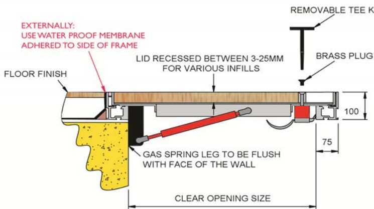
(Drawings show the access hatch recessed for oak flooring)
