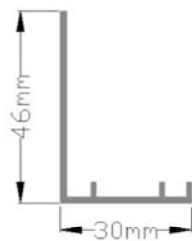
30mm flat flange
