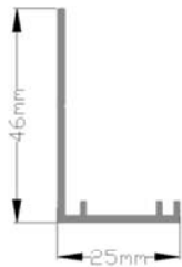
25mm flat flange
